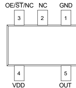
Figure 1. Pin Assignments
