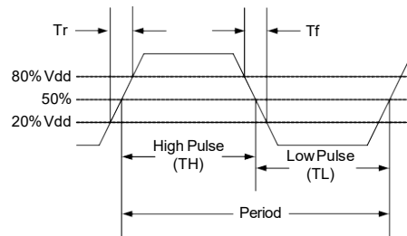
Figure 3. Output Waveform
