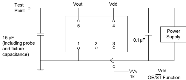
Figure 2. Test Circuit
