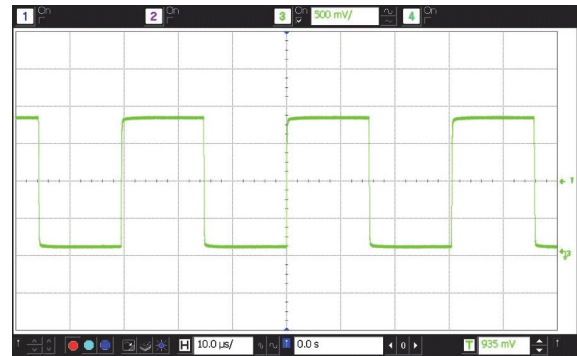
LVC MOS Output Waveform (V swing = 1.8V, TQC1532AI-J4-DCC-32.768)
