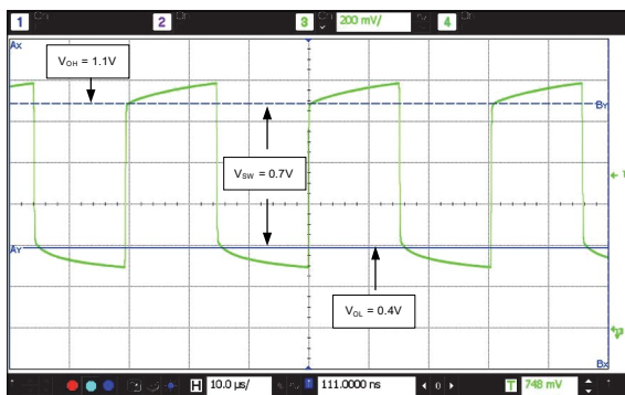
Figure 3. TQC1532AI-J4-D14-32.768 Output Waveform (10 pF load)
