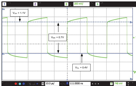
NanoDrive™ Output Waveform (V OH = 1.1V, V OL = 0.4V; TQC1532AI-J4-D14-32.768)
